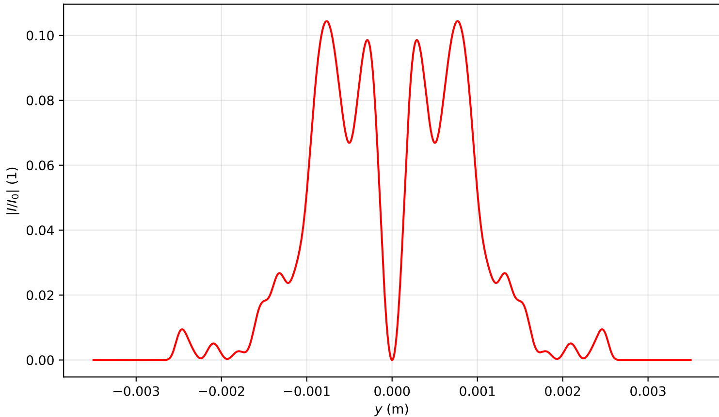
Intensity profile I(x=0, y, z=2.229)/I_0 , P_{in}=8.0P_{cr} , artificial time
